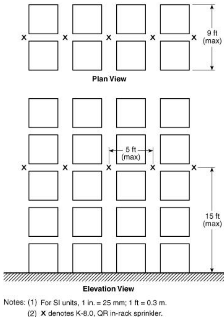
FIGURE 6.8.6.3(e) Double-Row Rack Sprinkler Layout.
